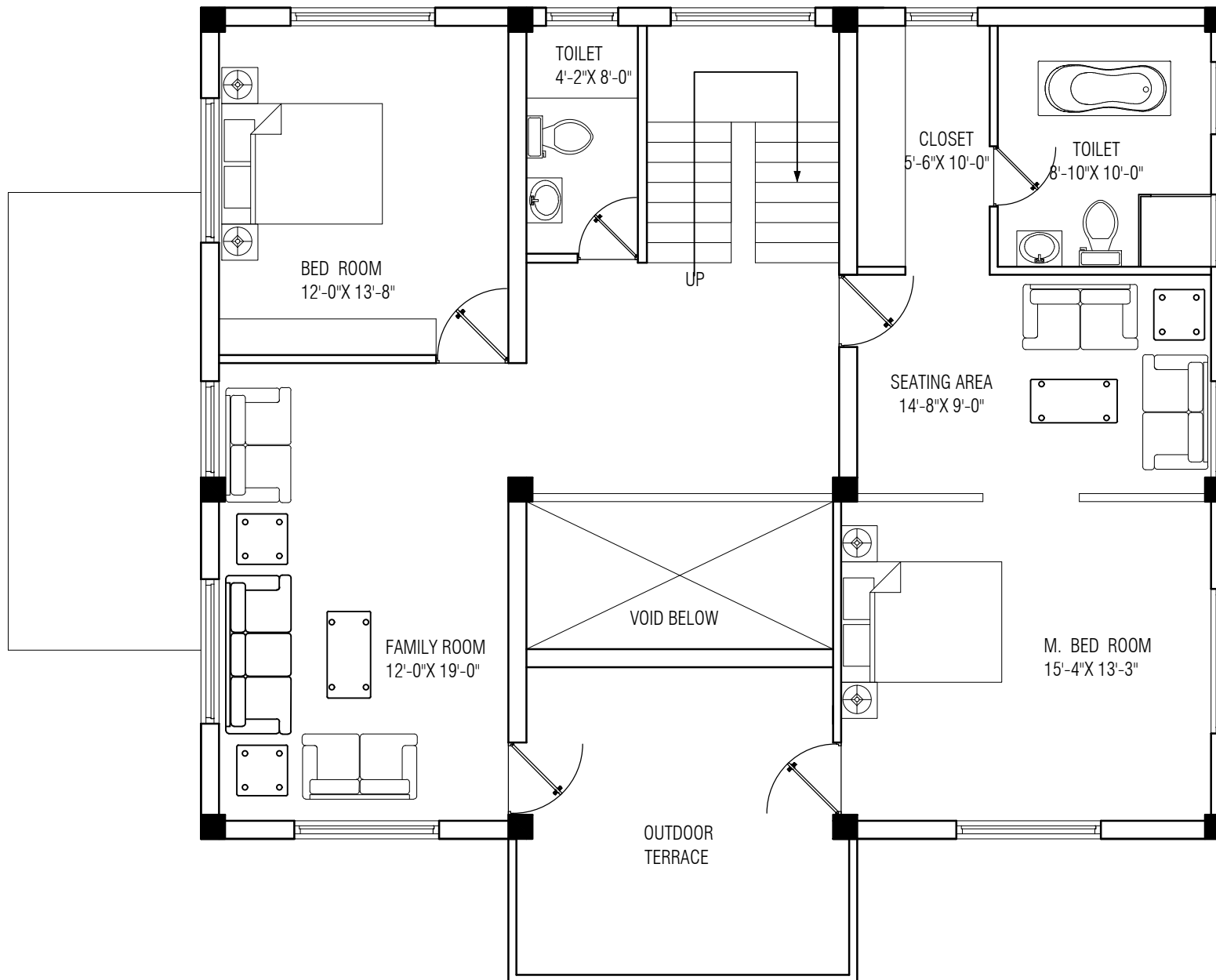
FIRST FLOOR PLAN Area: 1394 sq.ft
